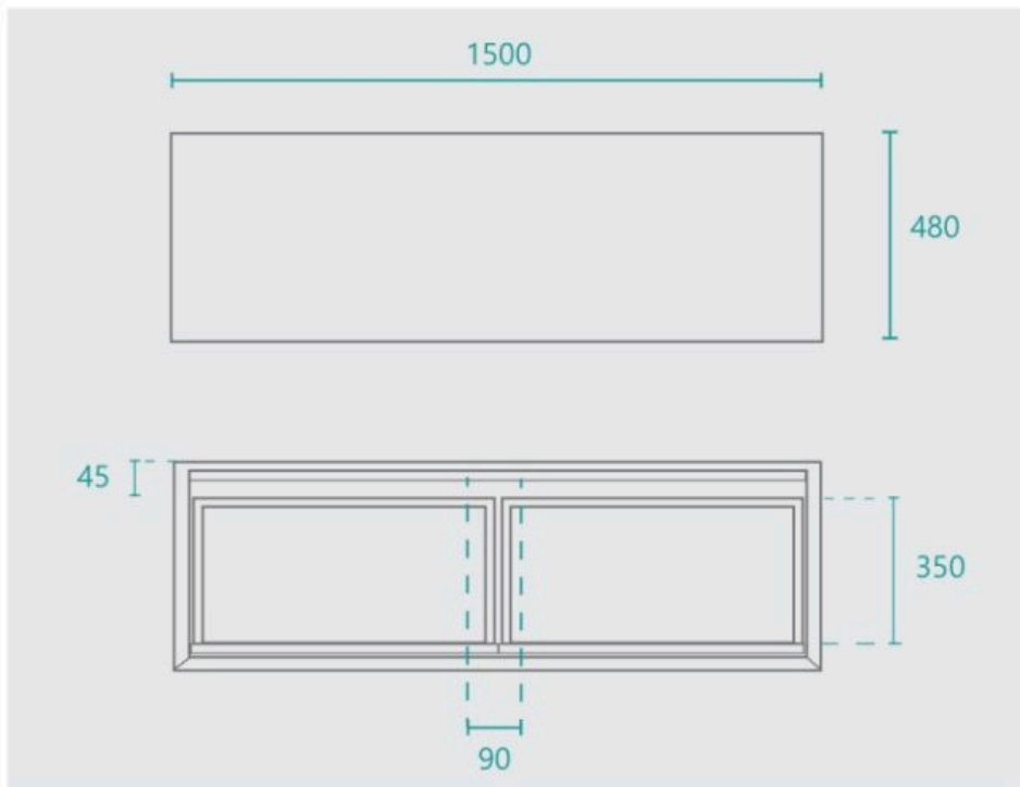
Paloma 1500 Wall Mounted Vanity
