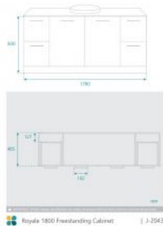
Royale 1800 Freestanding Cabinet | J-2043
