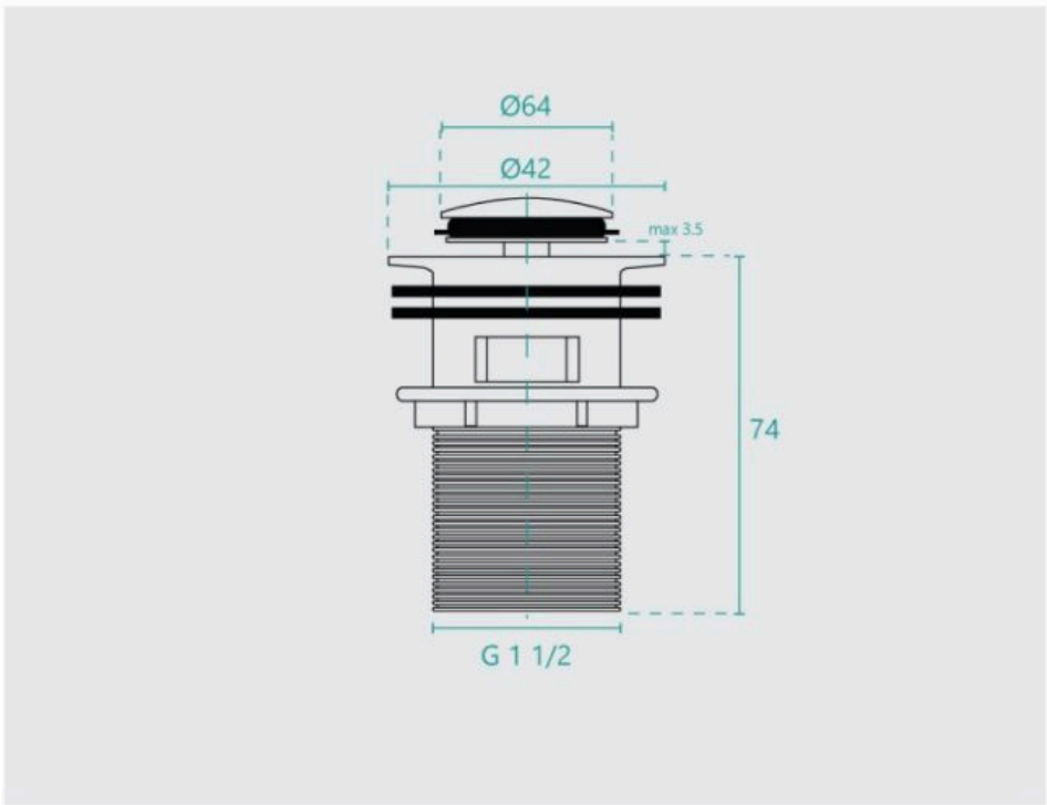
Waste Plug Pop Up 40mm Overflow
