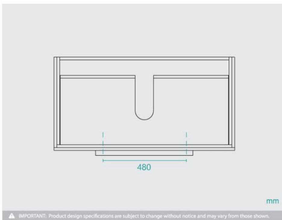
Handle Alloy 600 Black | HD-8006
